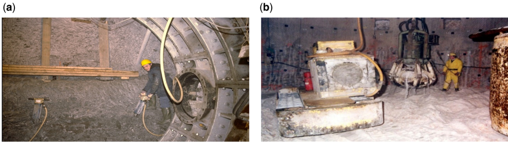
Fig. 16. (a) Manual excavation of the first gallery of the HADES URL in 1984 and (b) sinking of the shaft of the Gorleben URL in 1986. Source: (a) courtesy of ESV EURIDICE and (b) courtesy of BGE.
