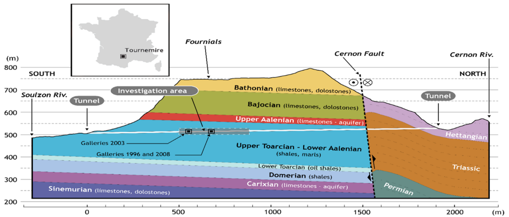
Fig. 4. The Tournemire URL uses an old railway tunnel excavated in clay. Source: modified from Matray et al. (2007), courtesy of IRSN.
