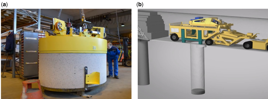
Fig. 17. POSIVA has used the ONKALO ® URCF to test their Buffer Installation Device: (a) prototype of the device and (b) drawing of the device in action in the ONKALO ® URCF. Source: POSIVA.
