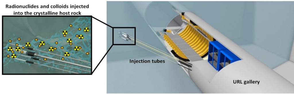
Fig. 10. The Colloid Formation and Migration project at the Grimsel Test Site, setup for the long-term in situ experiment. Source: courtesy of NAGRA.
