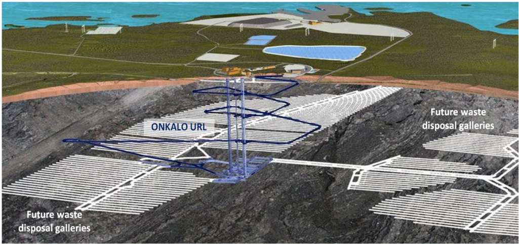
Fig. 3. The ONKALO® underground rock characterization facility (URCF) is a part of the access infrastructure to the current research facility and future disposal galleries. Source: POSIVA.
