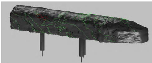
Fig. 7. Geological mapping data of fractures and lithological contacts in a niche in the ONKALO® URCF. Source: POSIVA.
